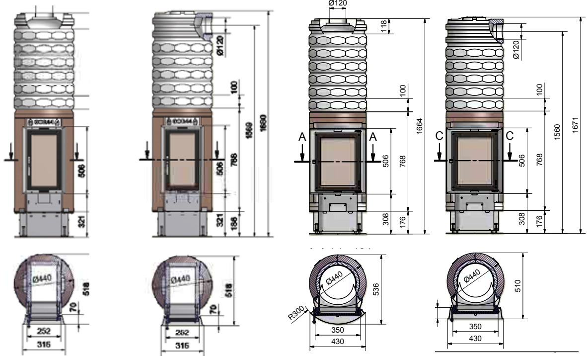
GOR44 Small doors
