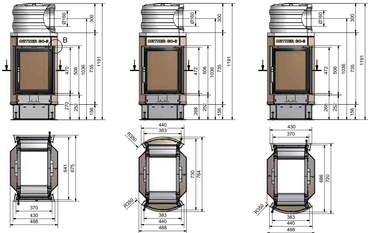
GO8T 2x straight doors 2x straight bezel
