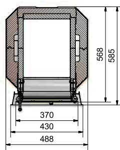
GO8 straight doors straight bezel
