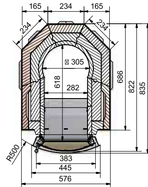
GO15 rounded doors rounded bezel
