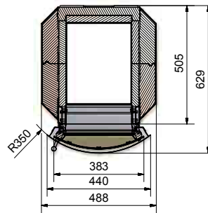
GO8 rounded doors rounded bezel
